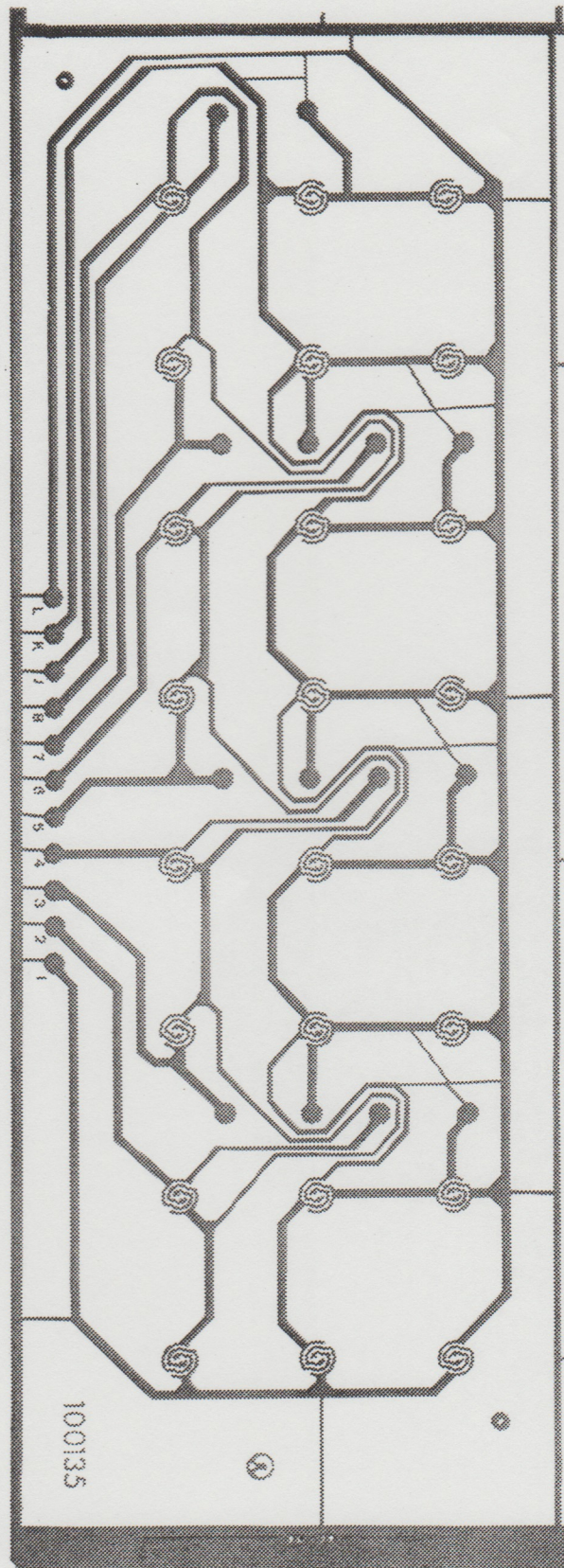
ART NO.909 SCRIPPO #100135 PCB - KEYBOARD
