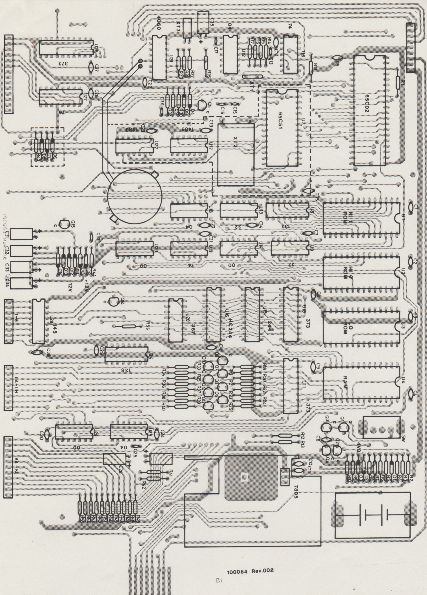
PCB LAYOUT #100084 component side with component location
